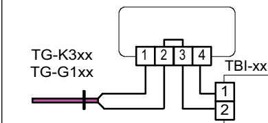
Figure 6: Wiring of external, separate sensor when using potentiometer TBI-xx as external setpoint
