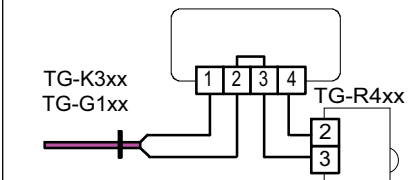
Figure 5: Wiring of external separate sensor when using TG-R4xx as external setpoint
