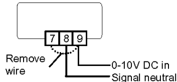
Abb 8: Externes Regelsignal
